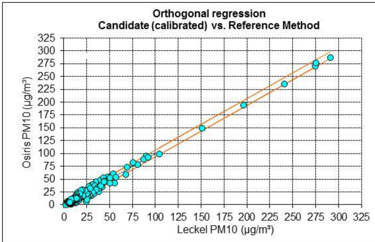
OSIRIS PM10 linearity
